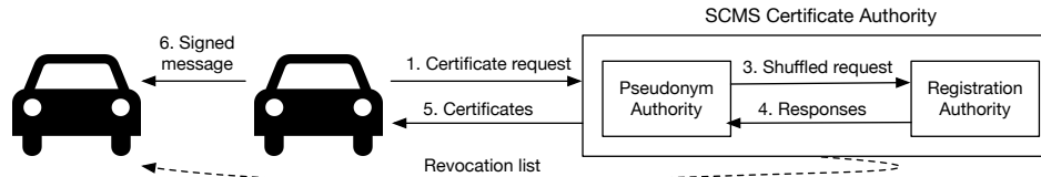
Figure 2: Overview of the SCMS Architecture
